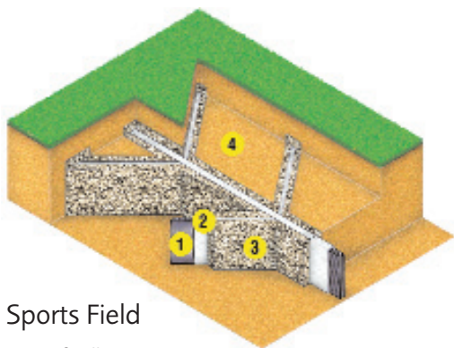
Capillary Irrigation
