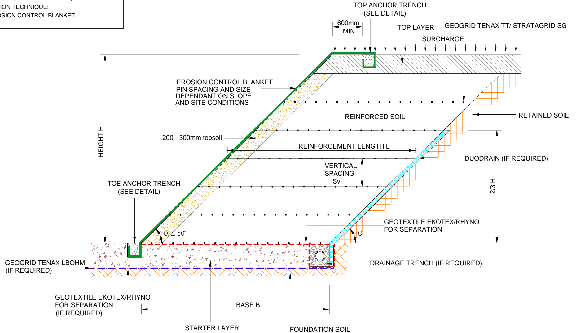
Cross-Section
