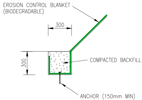
Toe Anchor Trench
