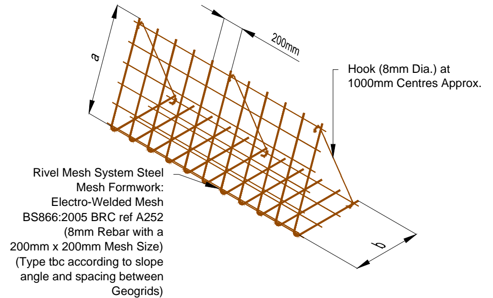
Rivel Mesh Formwork Detail
