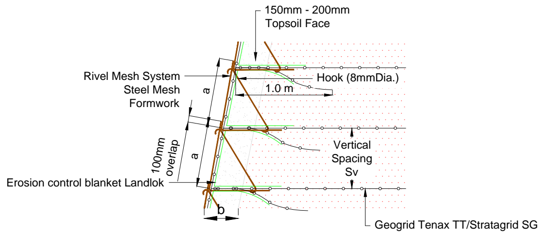
Wall Face Detail
